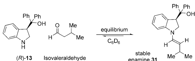
Scheme 8. ^1\text{H} NMR experiment to determine if the aldehyde is responsible for the decomposition of catalyst 13 during the reaction.
