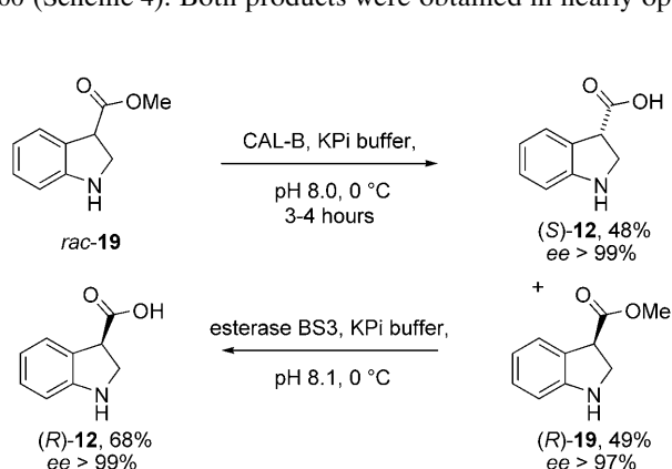
Scheme 4. Enzyme-mediated synthesis of ( R )- and ( S )-acid 12 .
