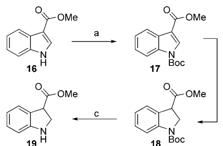
Scheme 3. Synthesis of rac - 19 . Reagents and conditions: a) NaH, Boc 2 O, THF, 95%; b) Mg turnings, MeOH, 93%; c) TFA, CH 2 Cl 2 , 97%.
