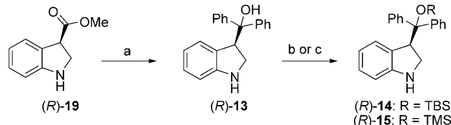
Scheme 6. Synthesis of diphenylcarbinols 13–15 . Reagents and conditions: a) PhMgBr, Et 2 O, 51 %; b) TBSTf, 2,6-lutidine, CH 2 Cl 2 , 83 %; c) TMSTf, 2,6-lutidine, CH 2 Cl 2 , 86 %.
