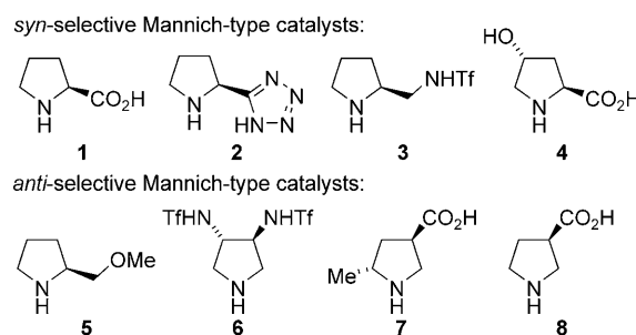
Scheme 1. Organocatalysts successfully employed in the Mannich type reaction.
