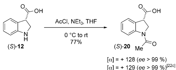
Scheme 5. Determination of the absolute configuration by means of chemical correlation.
