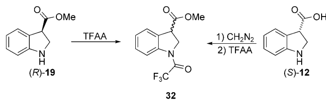
Scheme 9. Derivatization of acid ( S )- 12 and ester ( R )- 19 .
