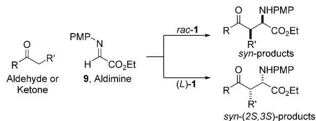
Scheme 7. Synthesis of syn Mannich bases catalysed by 1 .
