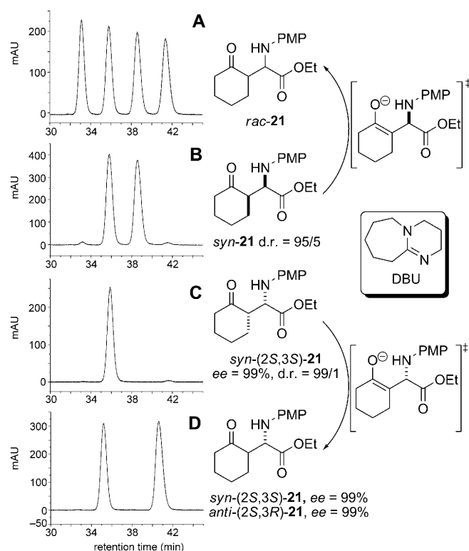
Figure 1. Representative procedure for the determination of the absolute configuration of the Mannich type reaction (controlled epimerisation of racemic syn - 21 and syn -(2 S ,3 S )- 21 ; DBU as base) and corresponding HPLC traces (column: Chiralpak IA (Daicel) [length: 25 cm, average internal diameter: 0.46 cm], flow rate: 0.5 mL min -1 , eluent: n -heptane/2-PrOH (92/8); R t [(2 R ,3 S )- 21 ]=33.1 min, R t [(2 S ,3 S )- 21 ]=35.8 min, R t [(2 R ,3 R )- 21 ]=38.6 min, R t [(2 S ,3 R )- 21 ]=41.4 min). A : racemic mixture of all diastereomers [ rac - 21 ] after epimerisation; B : syn diastereomers of compound 21 prepared with rac - 1 ; C : enantiopure (2 S ,3 S )- 21 prepared with ( S )- 1 ; D : ~1:1 mixture of epimers (2 S ,3 S )- 21 and (2 S ,3 R )- 21 , after epimerisation.
